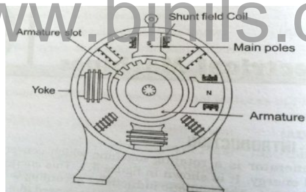
Figure 3.1.1 Construction of DC Motor
