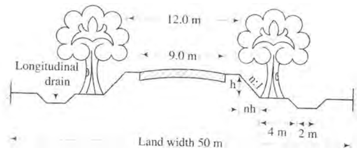
1.3.3.2 (c) Cross section of two lane national highway
