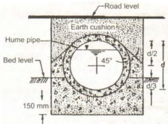
Fig. 5.3 Pipe culvert with Hume pipe
