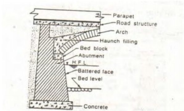
Fig. 5.24 Abutment for masonry arch bridge
