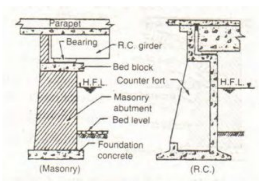
Fig. 5.26 Abutment for girder bridges
