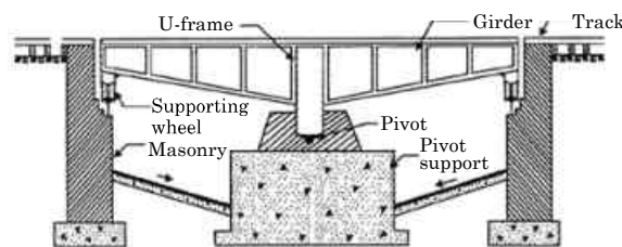
Fig.4.8 Turn table
