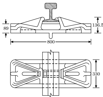
Fig.3.11 Cast-iron plate sleeper
