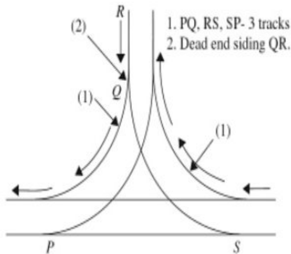
Fig.4.7 Triangle
