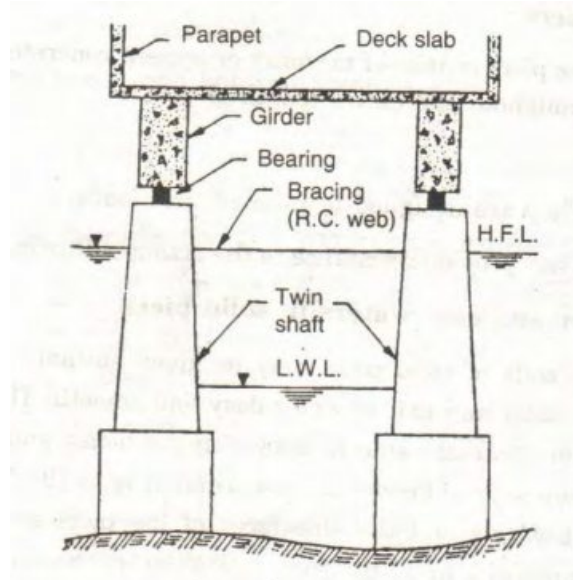
Fig. 5.18 Dumb-bell pier
