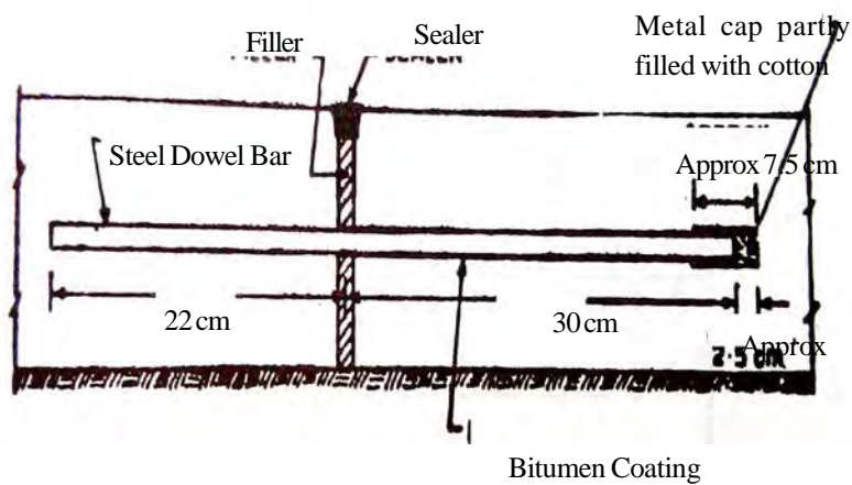
Fig. 2.5.6.2(i) Expansion Joint with Dowel Bar
