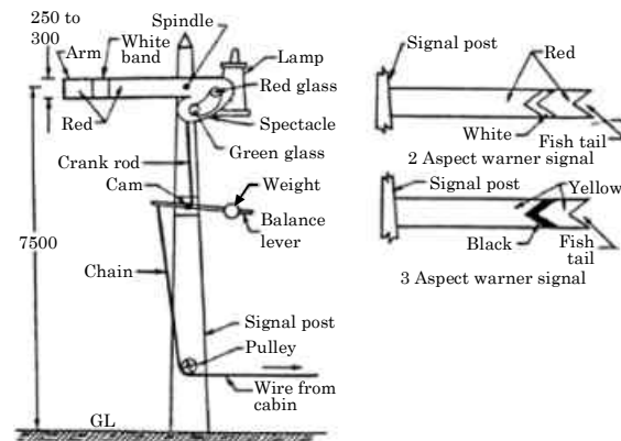
Fig.4.18 Semaphore and warner signal
