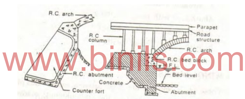
Fig. 5.25 Abutment for R.C. arch bridge
