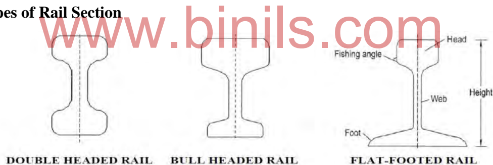
Fig.3.4 Rail sections
