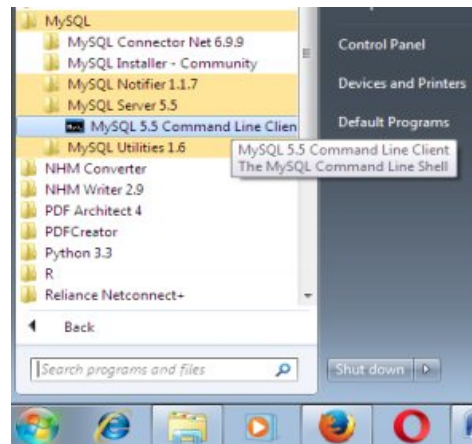
Fig. 2.1 Starting MySQL
