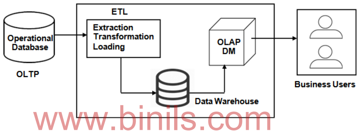
Fig. 1.7 - Decision Support Database
