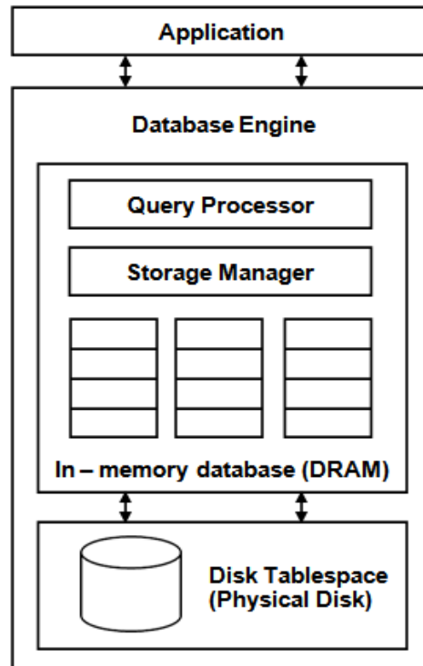
Fig. 1.8 - Hybrid Database
