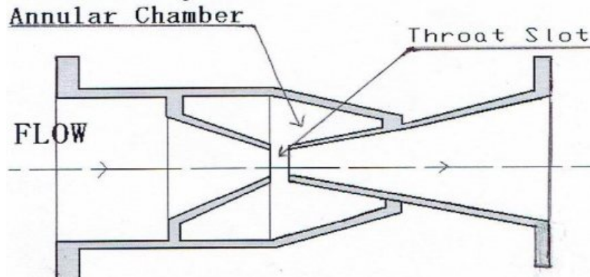
Fig 3.12 Dahl Tube
