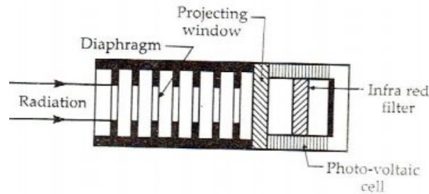
Fig 1.33 Infra-red Pyrometer
