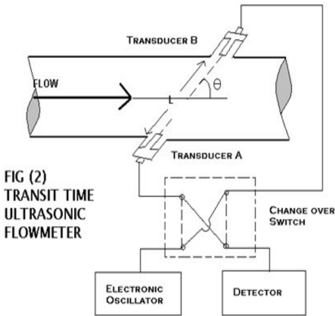
Fig 4.2 Transit Time Ultrasonic Flow meter
