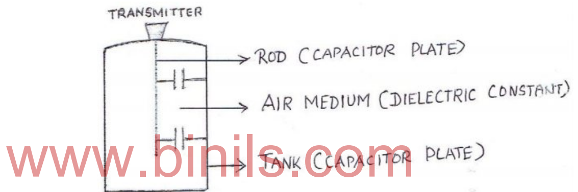
Fig 5.12 Basic method of Capacitance Level transducer
