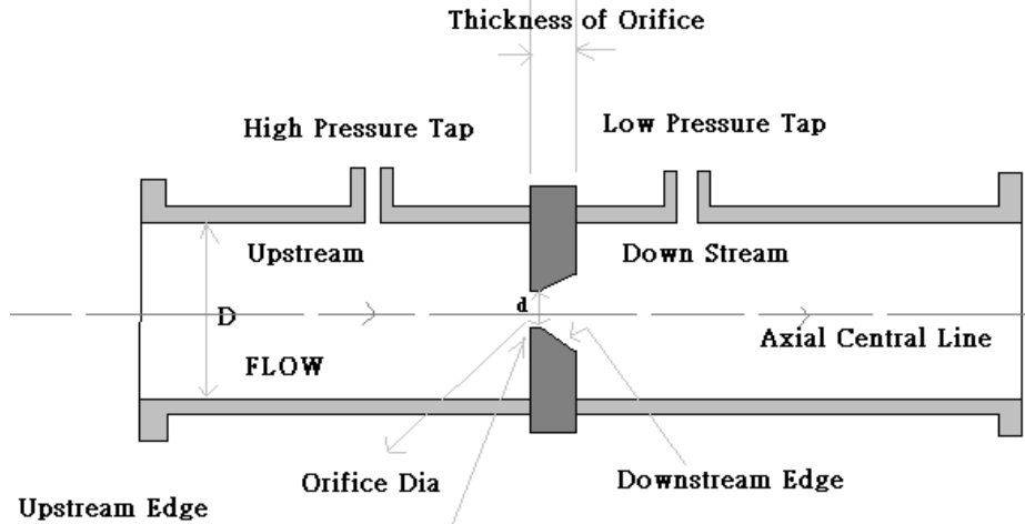
Fig 3.8 Orifice Plate Flow Meter
