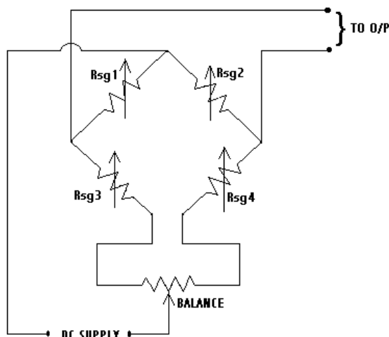
Fig 2.10 Strain Gauge Bridge Circuit
