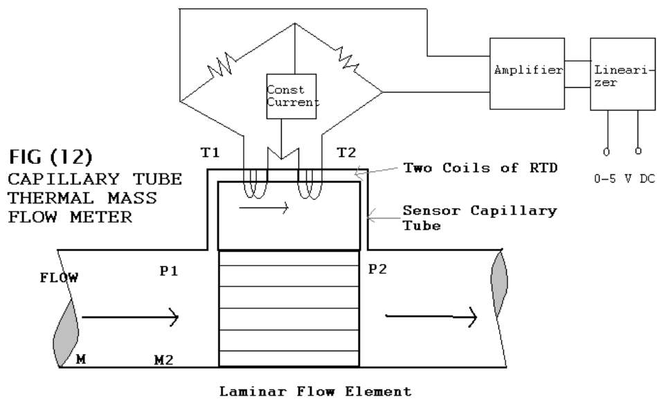
Fig 4.11 Capillary Tube Thermal Mass Flow Meter
