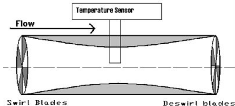
Fig 4.4 Swirl Flow Meter
