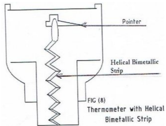
Fig 1.7 Bimetallic Thermometer with spiral strip Fig 1.8 Bimetallic Thermometer with helical strip change in temperature and 1/\text{thickness} of the metal strip. The movement of the bimetallic strip is utilized to deflect the pointer over a calibrated scale.
