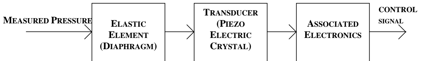
Fig 2.15 Block Diagram for Piezo Electric Pressure Transducer
