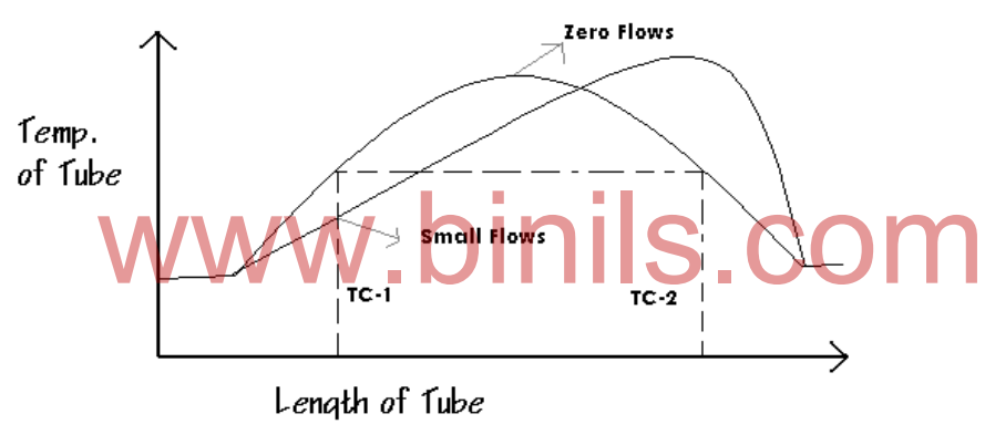
Fig 4.10 Temperature distribution under static and flowing conditions
