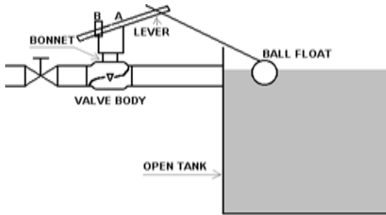
Fig 5.3 Float Valve
