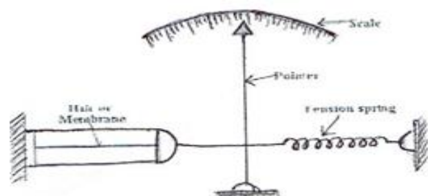
Fig 5.29 Hair Hygrometer
