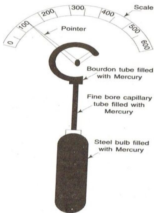
Fig 1.2 Mercury in Steel Thermometer
