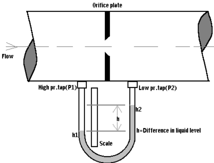
Fig 2.1 U-Tube Manometer
