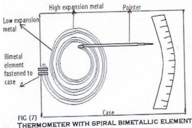
Fig 1.7 Bimetallic Thermometer with spiral strip Fig 1.8 Bimetallic Thermometer with helical strip change in temperature and 1/\text{thickness} of the metal strip. The movement of the bimetallic strip is utilized to deflect the pointer over a calibrated scale.
