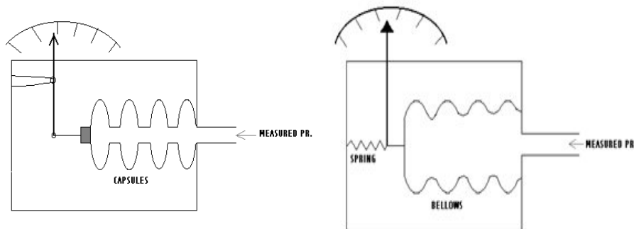
Fig 2.9 Gauge with Capsule and Bellows
