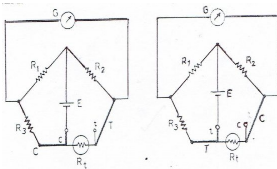
Fig 1.17 Four wire RTD system
