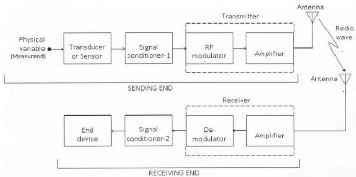
Fig 2.22 Block diagram of Radio frequency telemetry system
