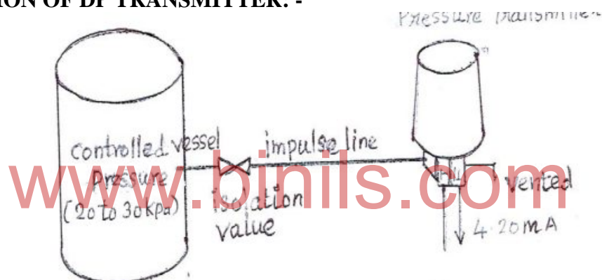
Fig 2.20 Installation of DP Transmitter
