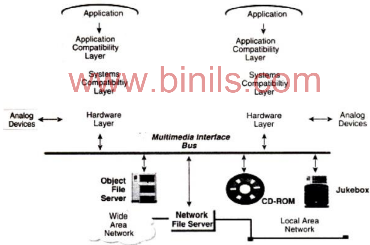
Fig 1.2. IMA Architecture
