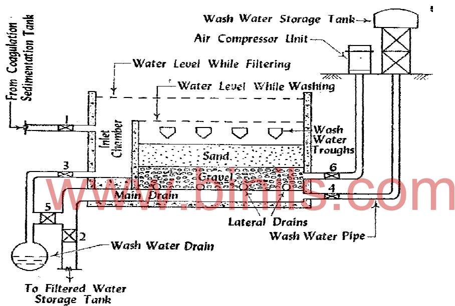
Fig 2.4(b) – Section of a typical rapid sand filter (gravity type)
