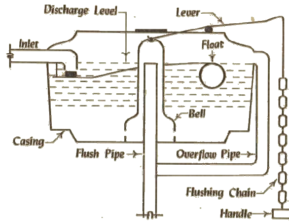
Flushing cisterns
