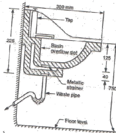
Wash basin
