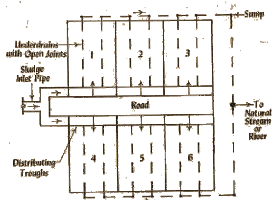
Plan of drying beds FIG. 14-1
