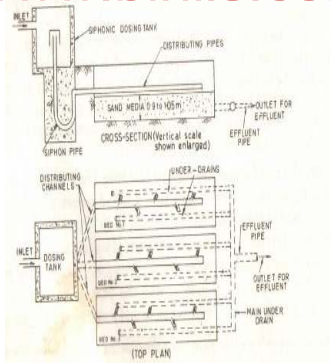
Intermittent sand filters
