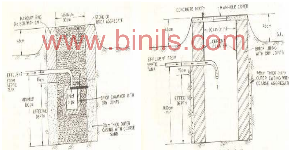
Unlined soak pit
