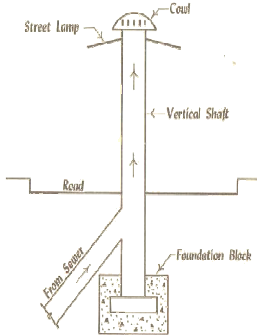
Ventilating columns
