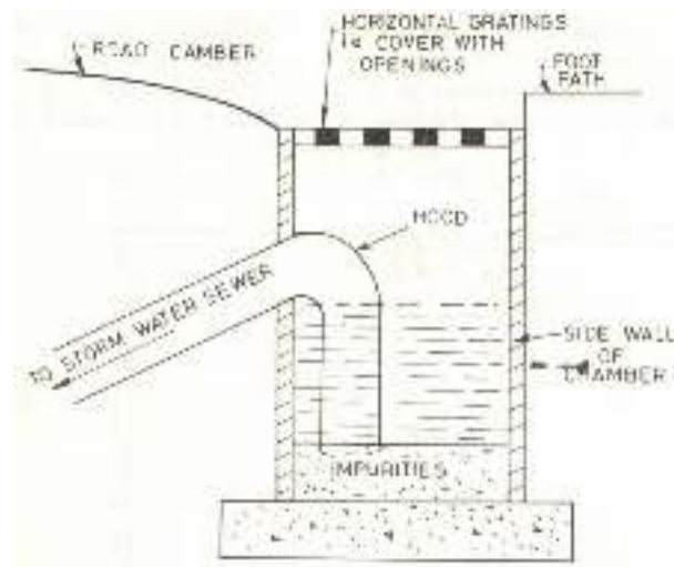
Catch basin
