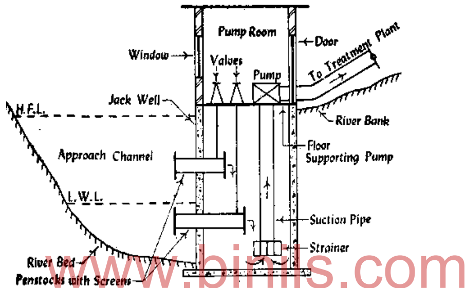
Fig 1.4 – River intake
