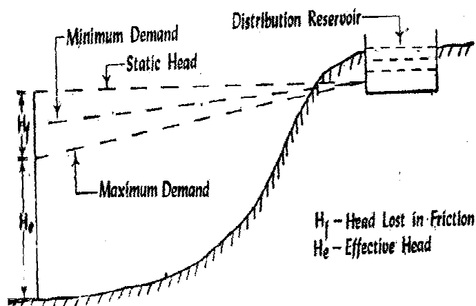
Fig 2.6 – Gravity System
