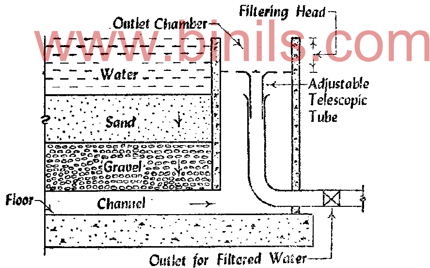
Fig. 2.3(b) – Cross – section through outlet chamber
