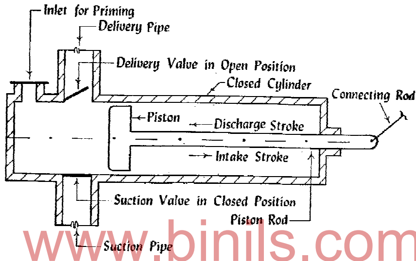
Fig 1.8 – Reciprocating pump
