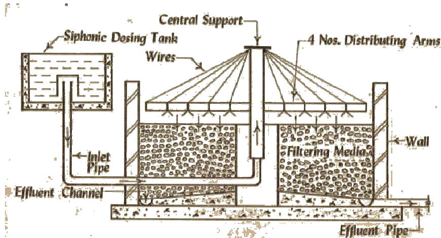
Trickling filter
