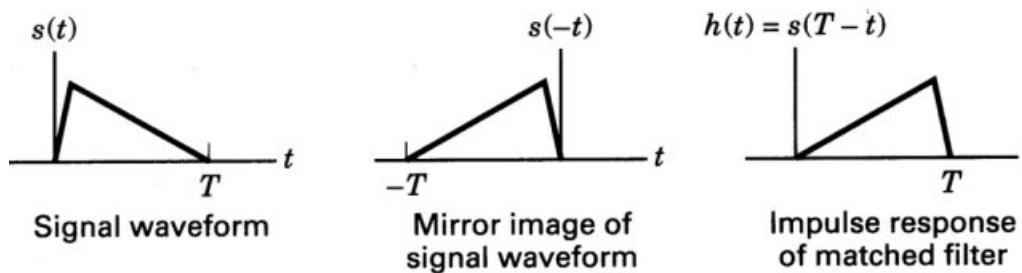
Figure 4.21 Matched filter characteristics
