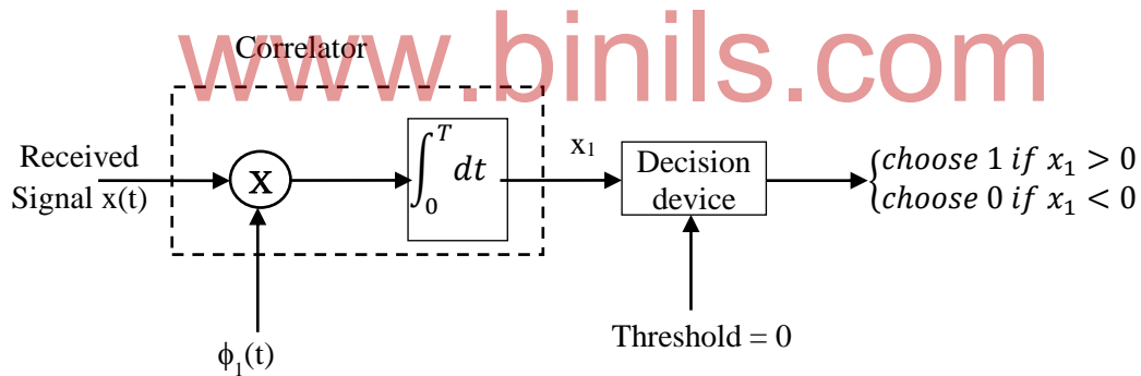
Figure 4.23 coherent binary PSK receiver
