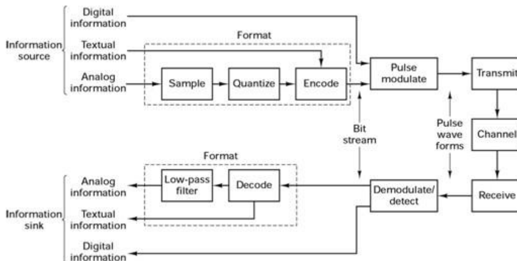
Figure 2.1 Formatting and Transmission of baseband signals (Baseband Systems)
