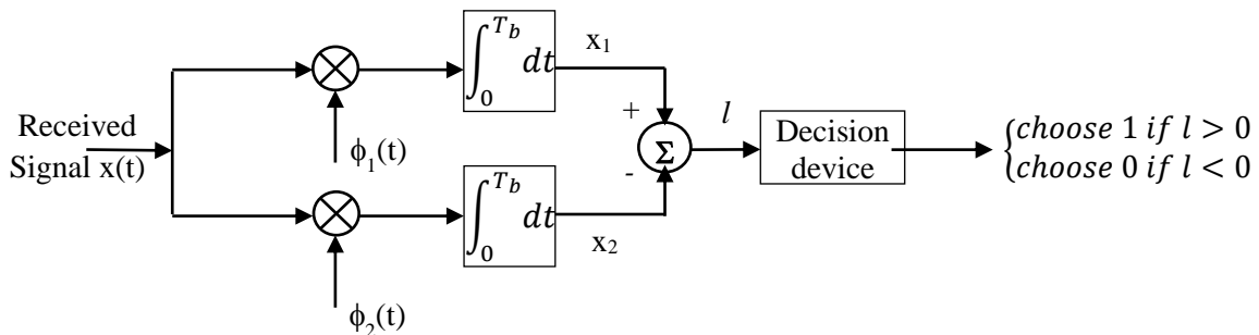
Figure 4.26 coherent binary FSK receiver
