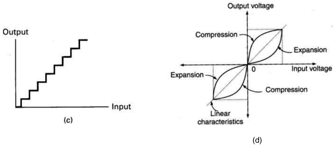
Figure 2.17 Non uniform Quantizer Characteristic
