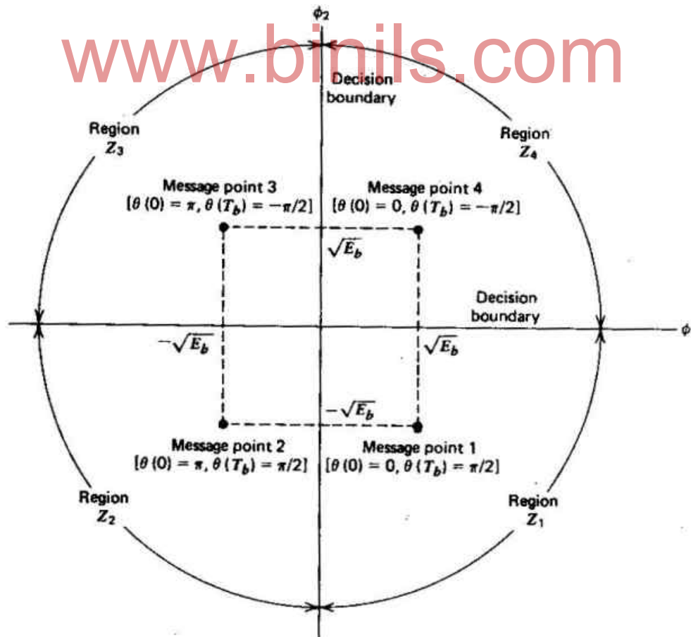
Figure 4.18 signal space diagram for MSK system
