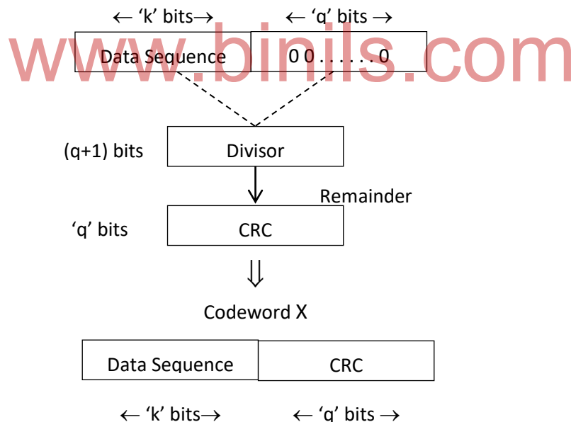
Figure 3.8 CRC Generation
