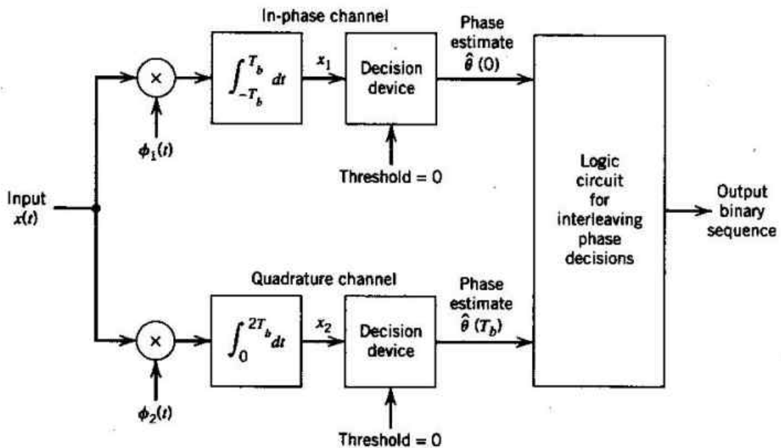
Figure 4.17 Block diagram of MSK receiver
