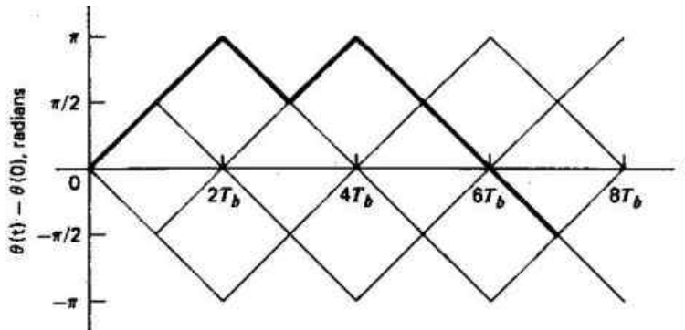
Figure 4.14 phase trellis (for the sequence 1101000)
