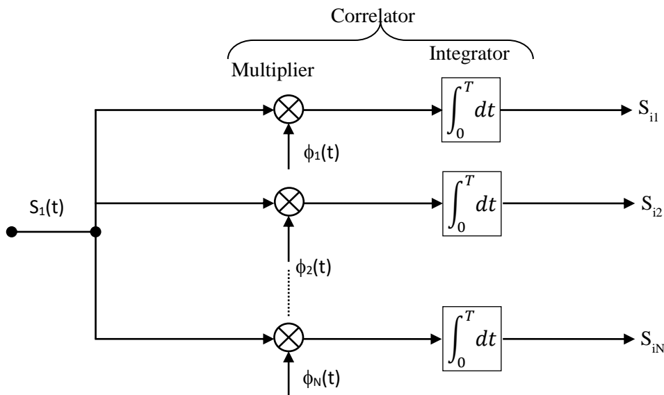
Figure 4.2 Scheme for generating the set of coefficients \{S_{ij}\}
