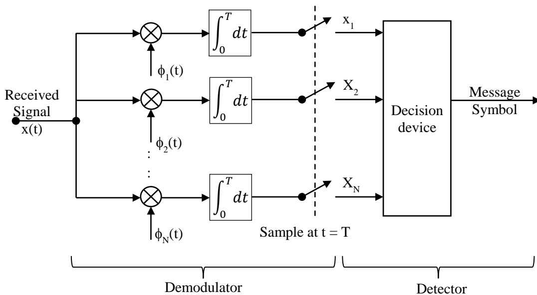
Figure 4.20 Correlator receiver
