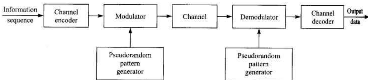
Figure 5.1 Model of spread spectrum digital communication system
