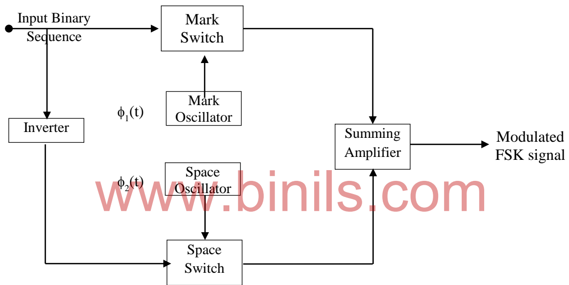
Figure 4.5 (b) BFSK Modulator
