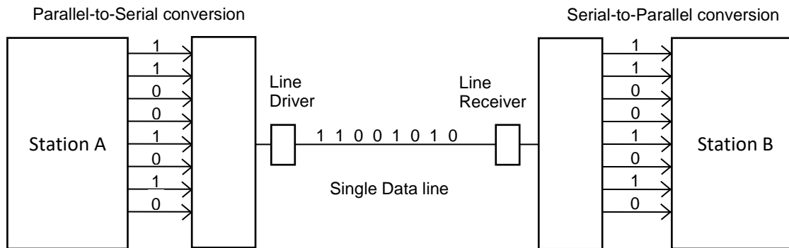
Figure 1.9 Serial Transmission
