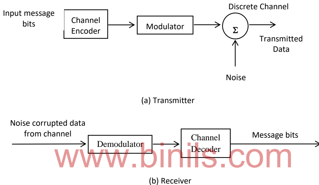
Figure 3.1 Digital Communication System with Channel Coding
