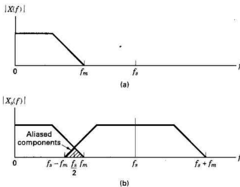
Figure 2.8 Aliasing in the frequency domain
