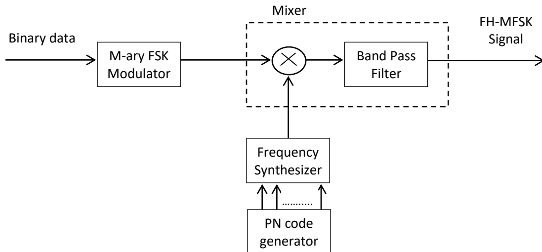
Figure 5.12 FH-MFSK Transmitter
