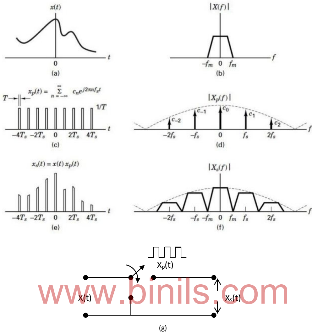
Figure 2.4 Natural Sampling
