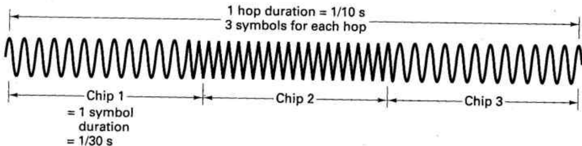
(b) Slow frequency hopping
