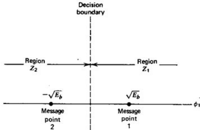
Figure 4.24 Signal-Space diagram for coherent BPSK
