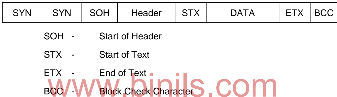
Figure 1.13 Character oriented Synchronous Protocol
