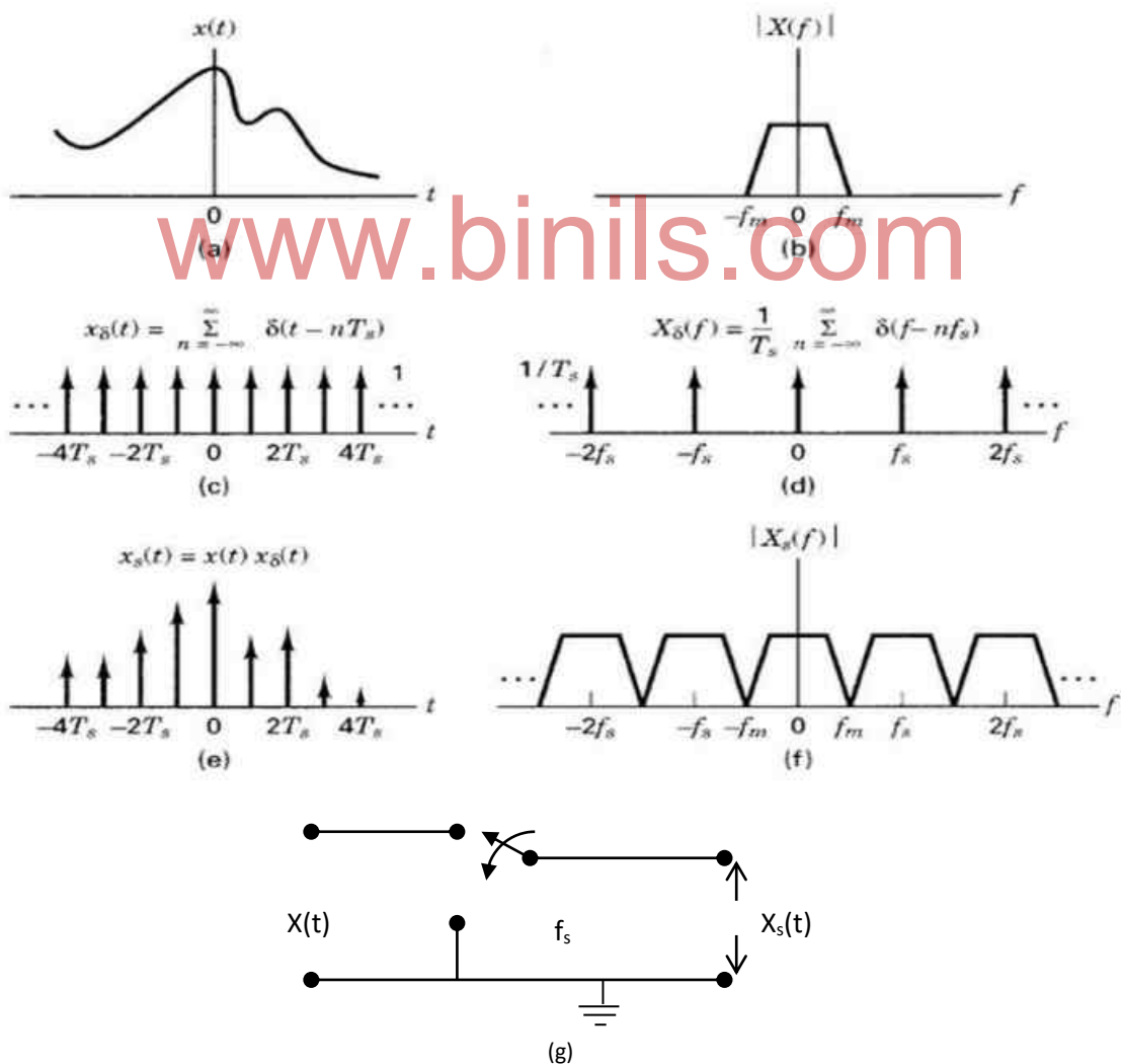
Figure 2.2 Impulse Sampling
