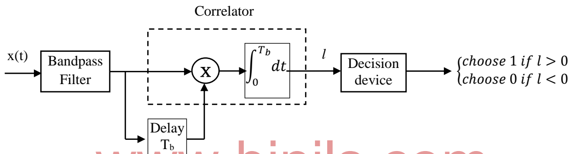
Figure 4.29 Non-coherent receiver for DPSK
