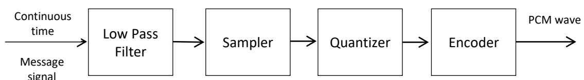
Figure 2.13 PCM transmitter
