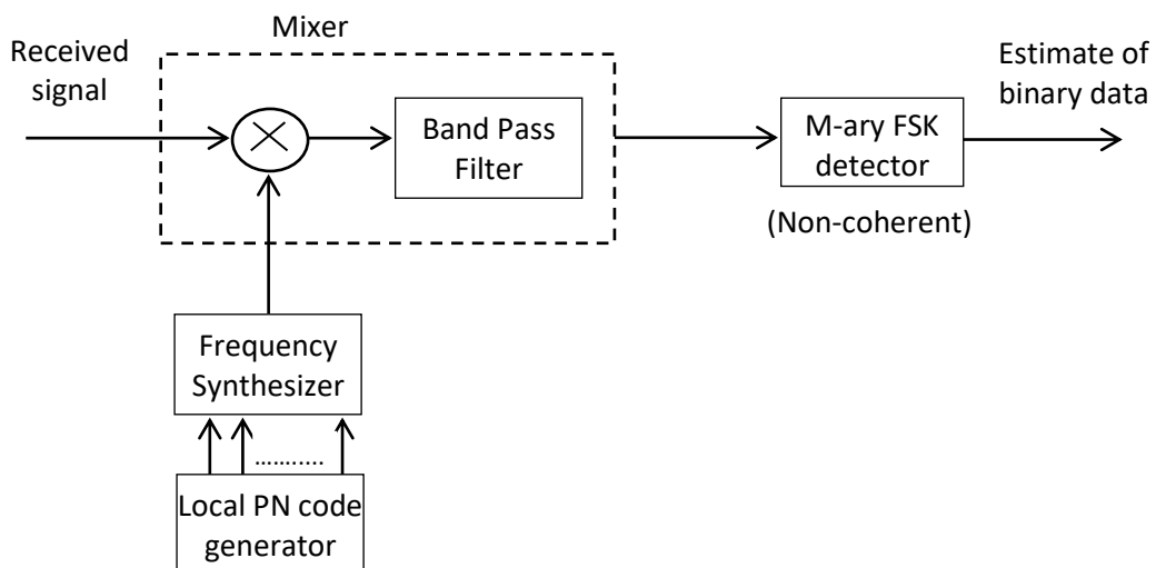
Figure 5.13 FH-MFSK Receiver
