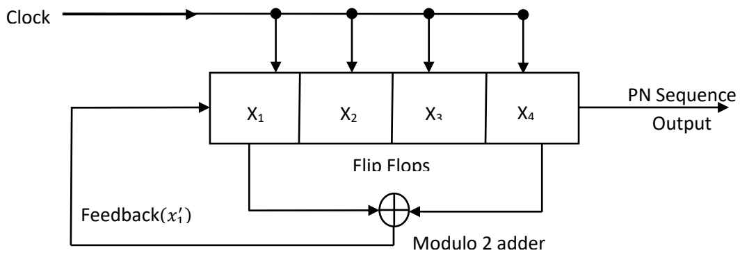
Figure 5.5 PN Sequence Generator
