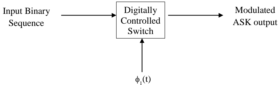
Figure 4.7 BASK Modulator
