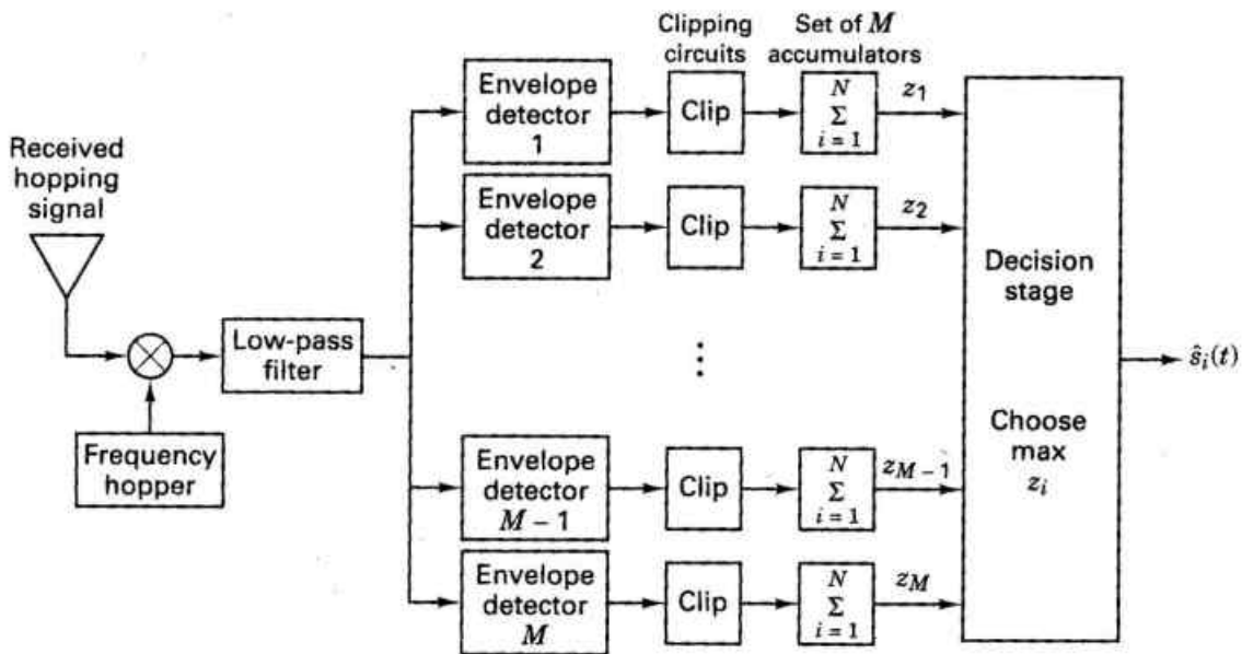
Figure 5.16 Fast FH-MFSK demodulator
