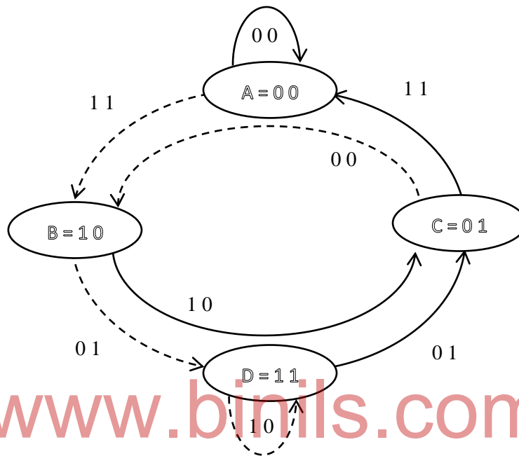
Figure 3.12 State diagram
