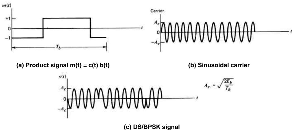
Figure 5.9 Waveforms for Second Stage of Modulation
