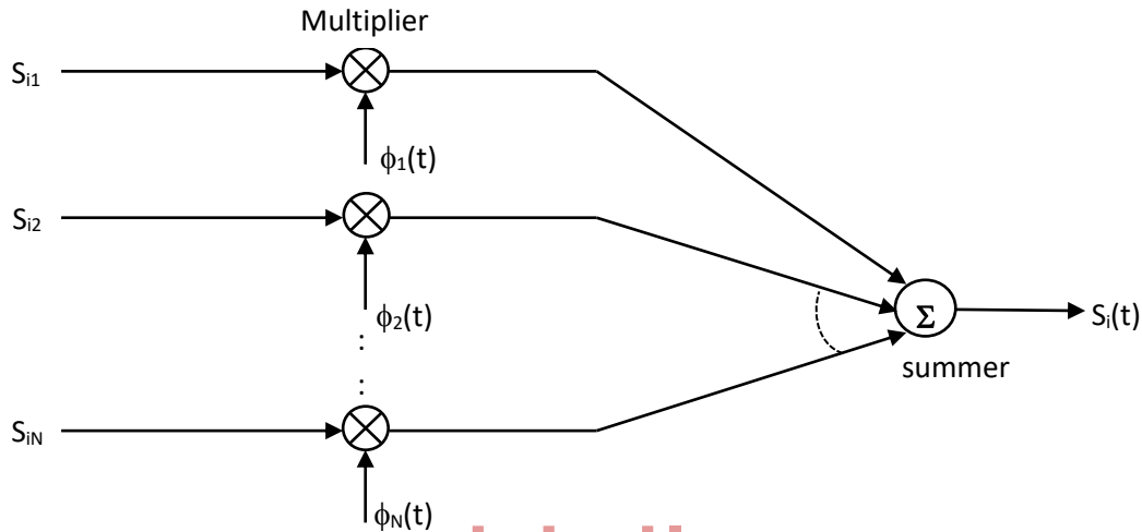
www.binils.com Figure 4.1 Scheme for generating the signal S_i(t)
