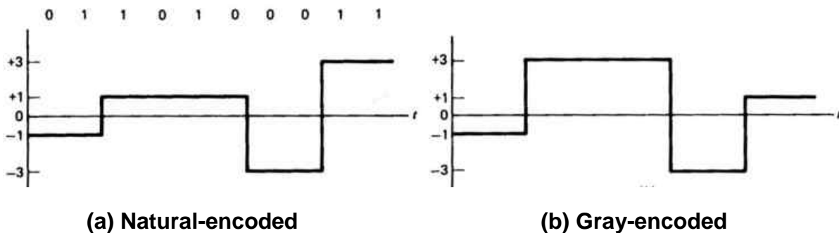
Figure 2.21 Polar Quaternary NRZ format
