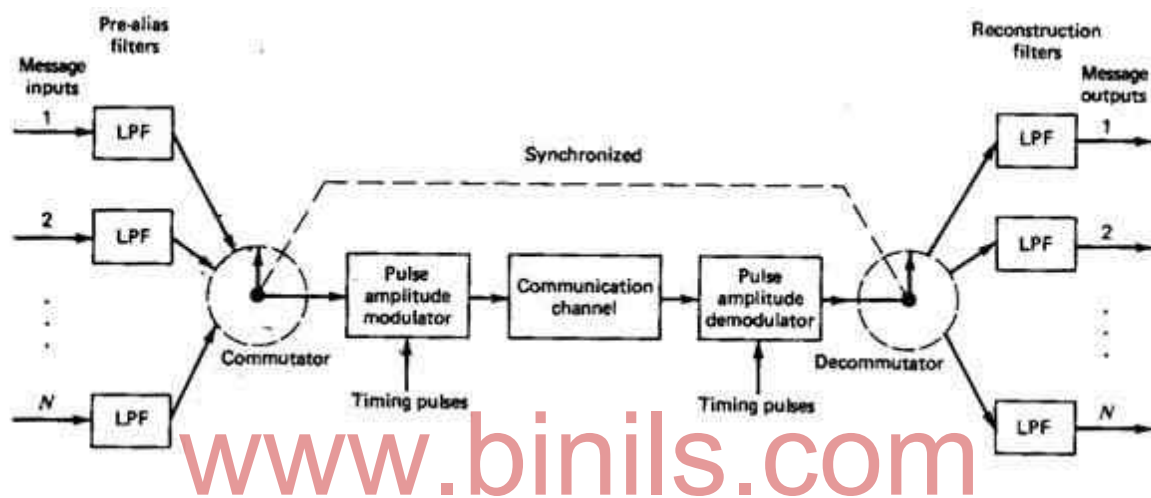
Figure 4.30 Block diagram of PAM / TDM system
