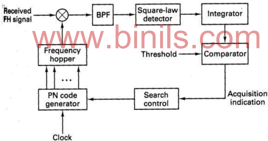
Figure 5.20 Frequency hopping serial search acquisition
