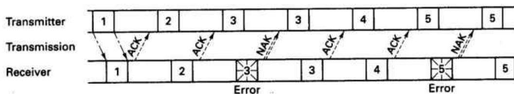
(a) Stop-and-wait ARQ
