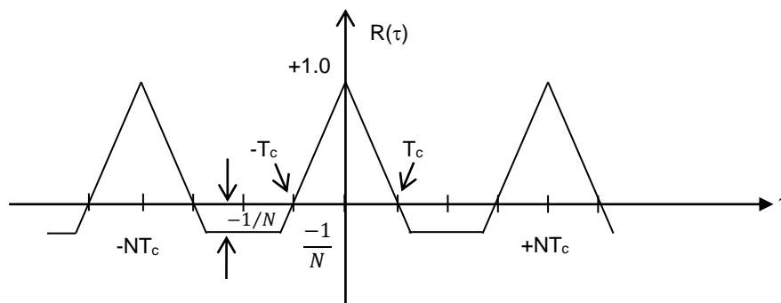
Figure 5.4 Autocorrelation function of a PN sequence
