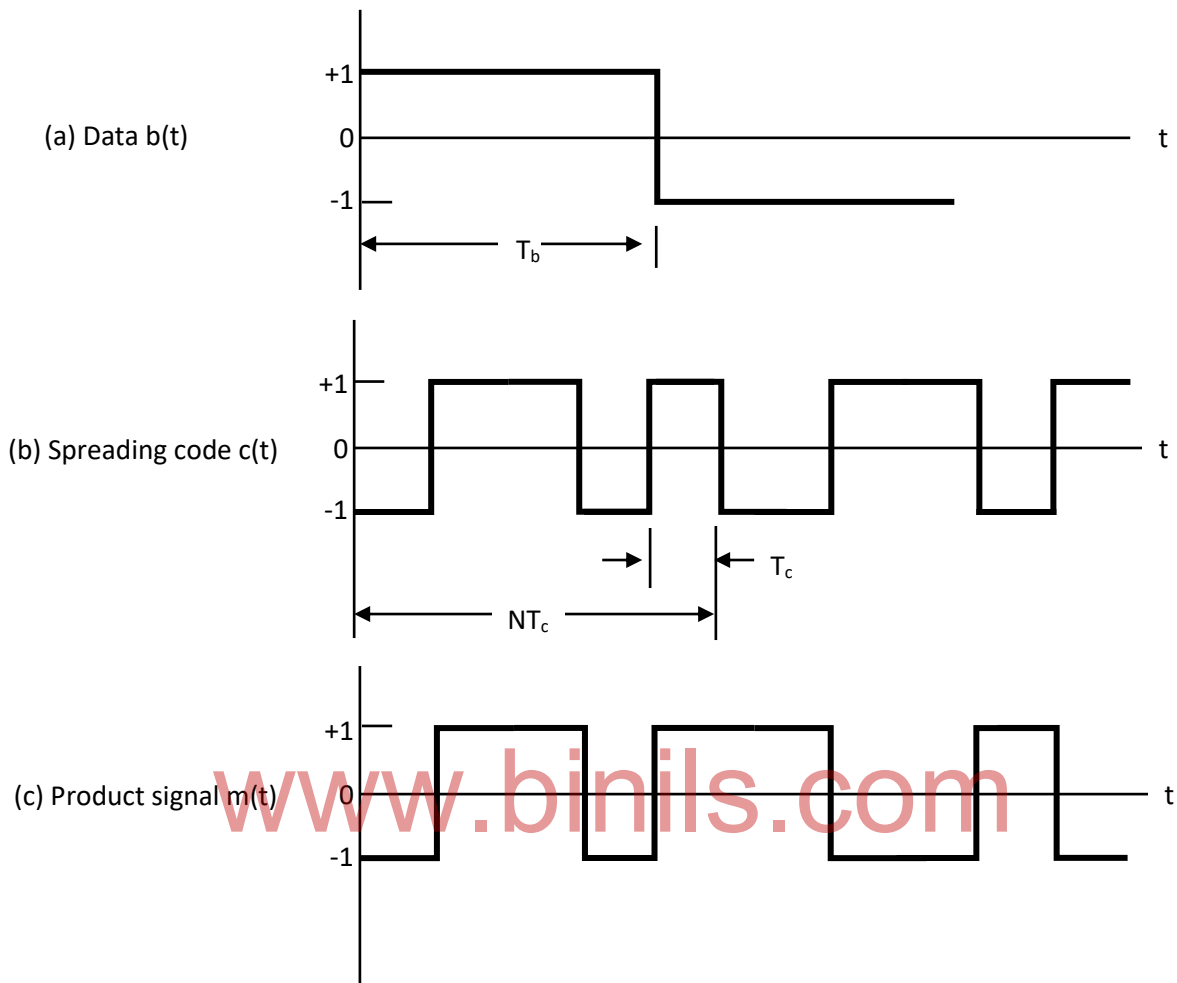
Figure 5.8 Waveforms for First stage of modulation
