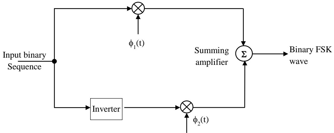
Figure 4.5 (a) BFSK Modulator
