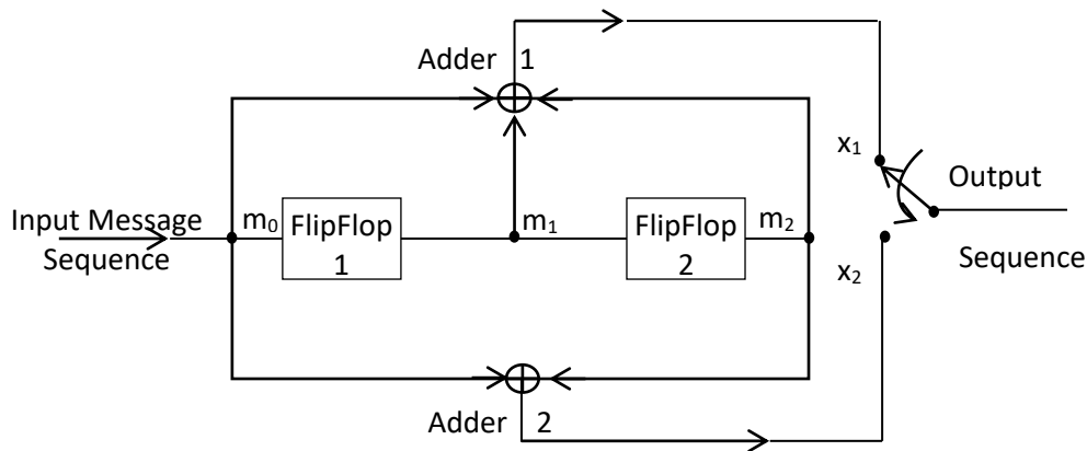
Figure 3.11 Convolutional Encoder Example
