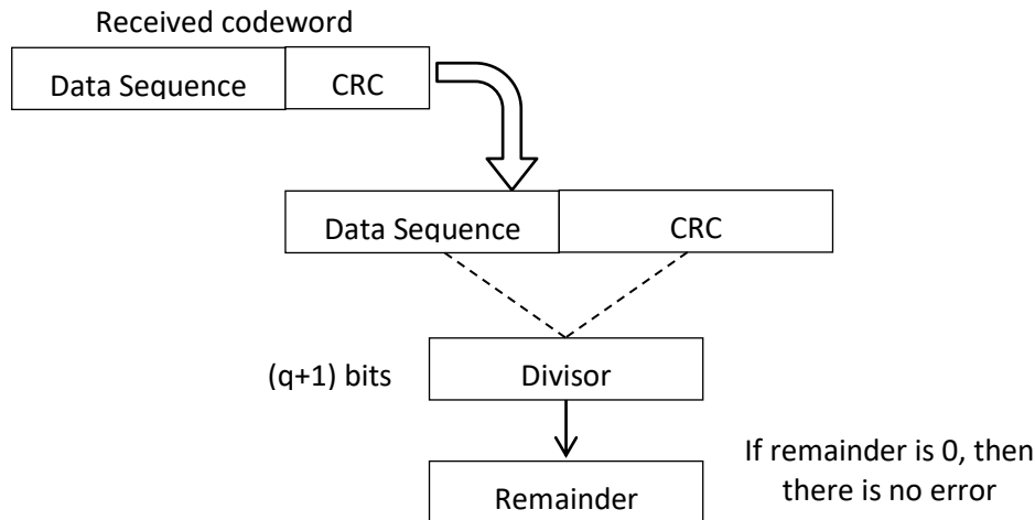
Figure 3.9 CRC checker
