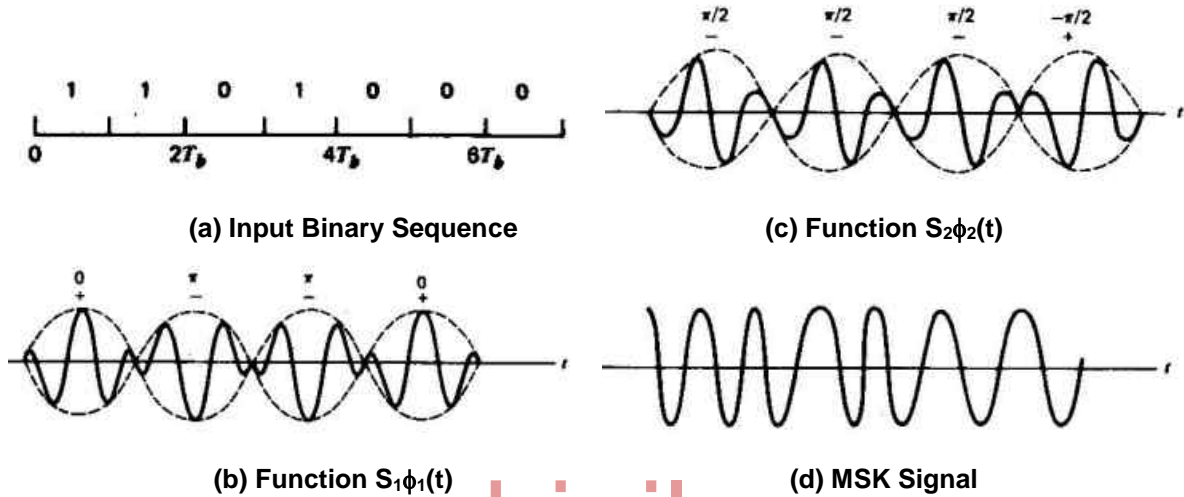
www.binils.com Figure 4.16 sequence and waveforms for MSK signal
