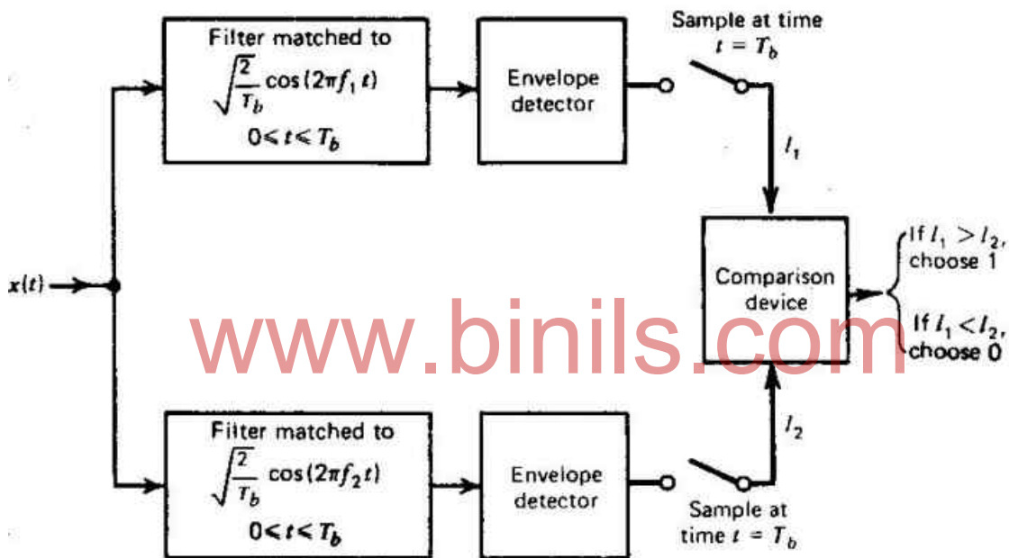
Figure 4.28 Non-coherent receiver for BFSK Digital communications
