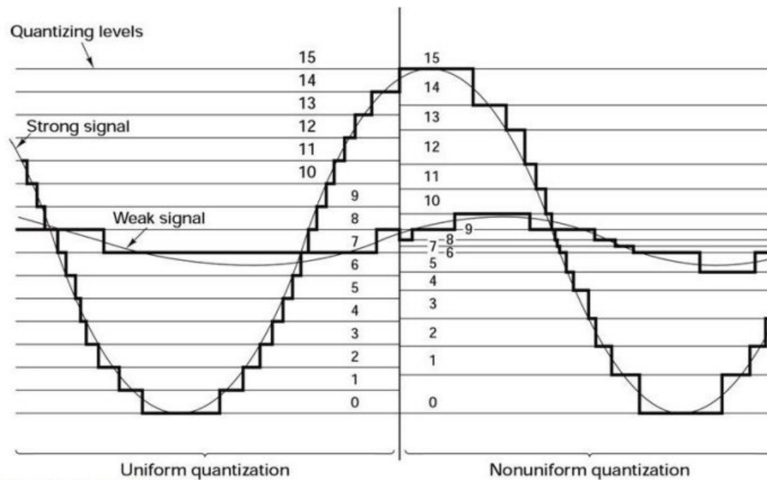
Figure 2.19 Performance Comparison
