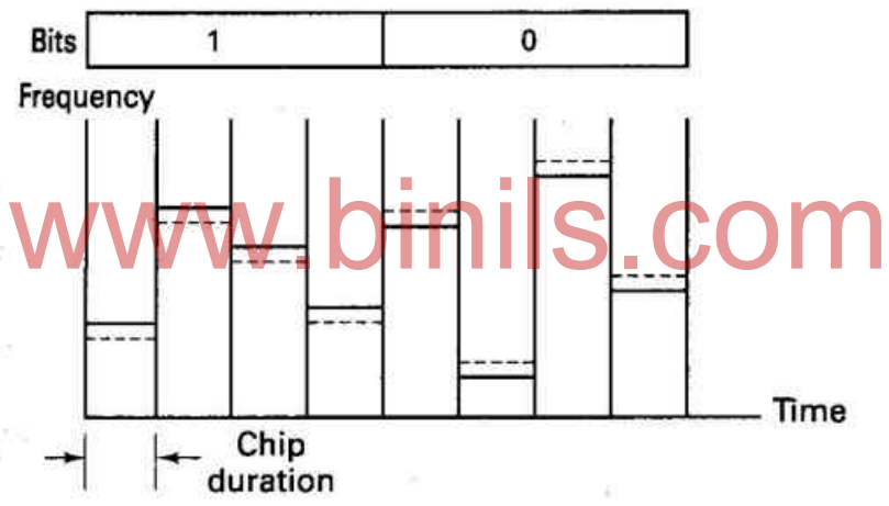
(a) Fast Frequency Hopping
