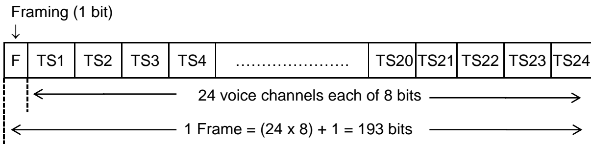
Figure 4.37 T1 Framing format
