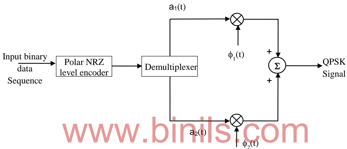
Figure 4.9 QPSK Transmitter
