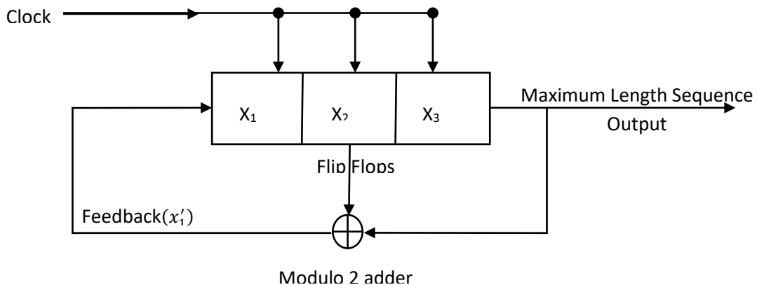
Figure 5.2 PN sequence or Maximum Length Sequence Generator
