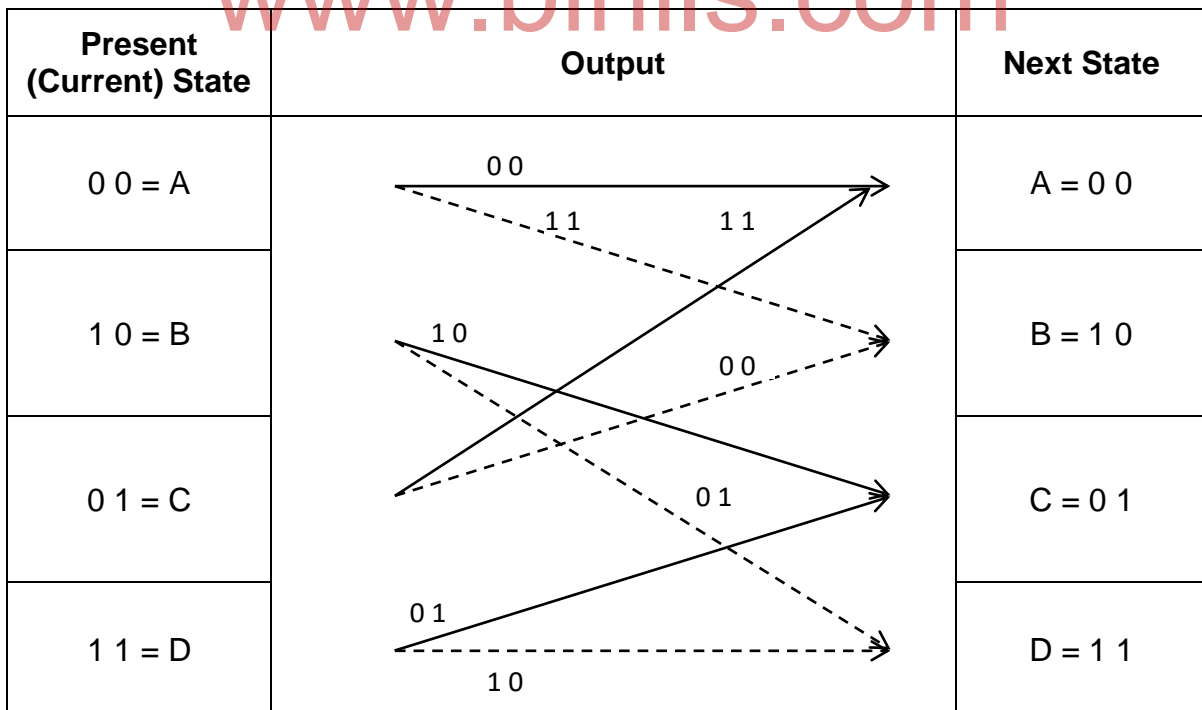
Fig.3.14 Code Trellis
