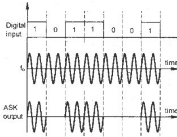
Figure 4.8: Wave forms for BASK
