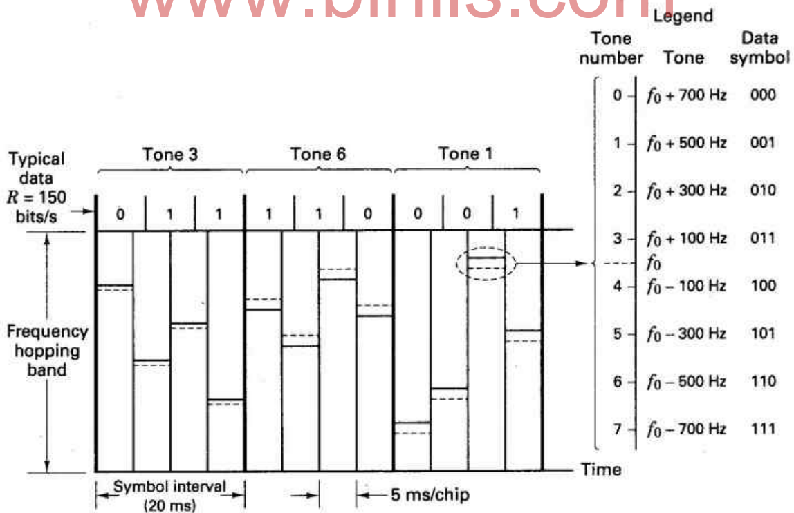
Figure 5.15 Frequency hopping with diversity (N = 4)
