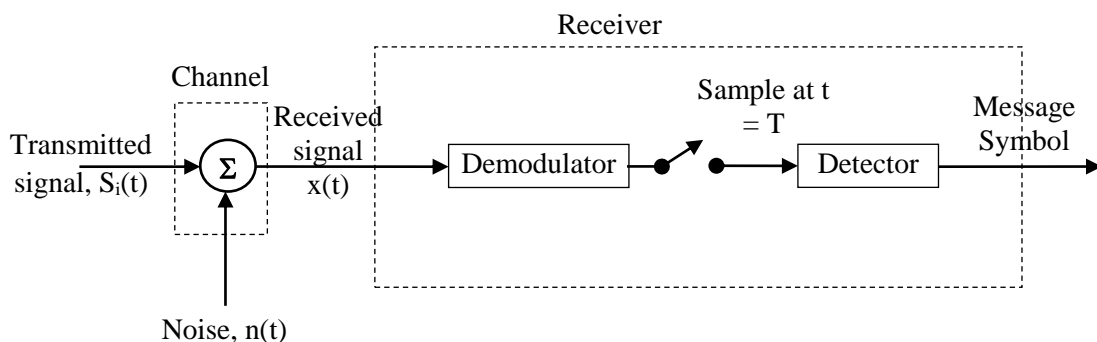
Figure 4.19 Two basic steps in digital receiver
