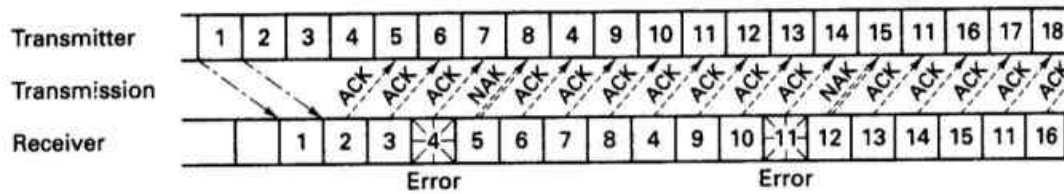
(c) Selective repeat ARQ
