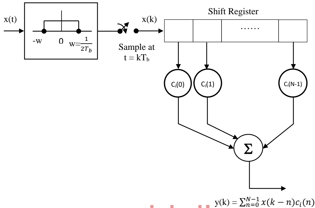
Figure 4.25 Sampled matched filter
