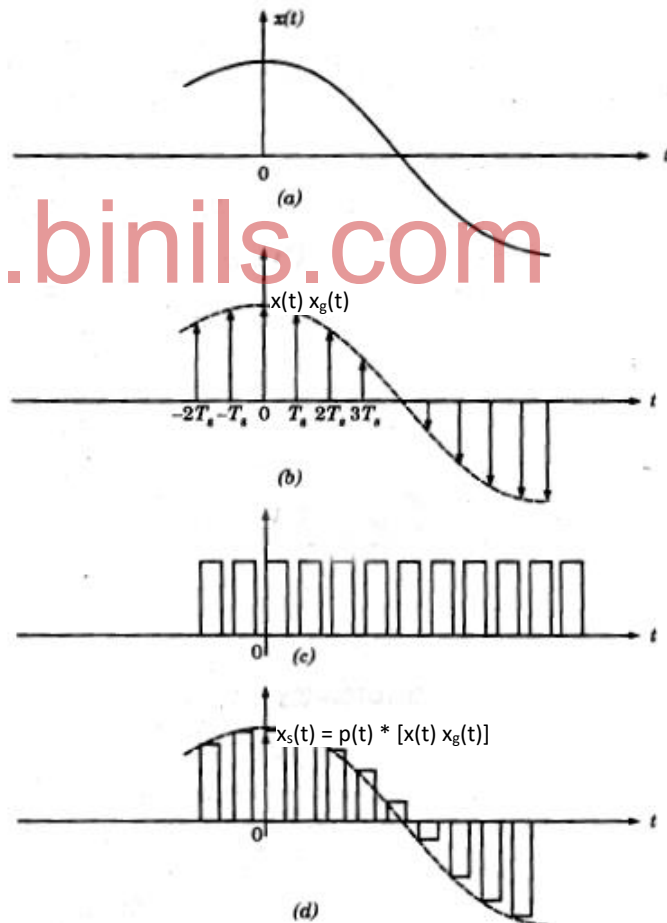
Figure 2.6 Flat Top Sampling
