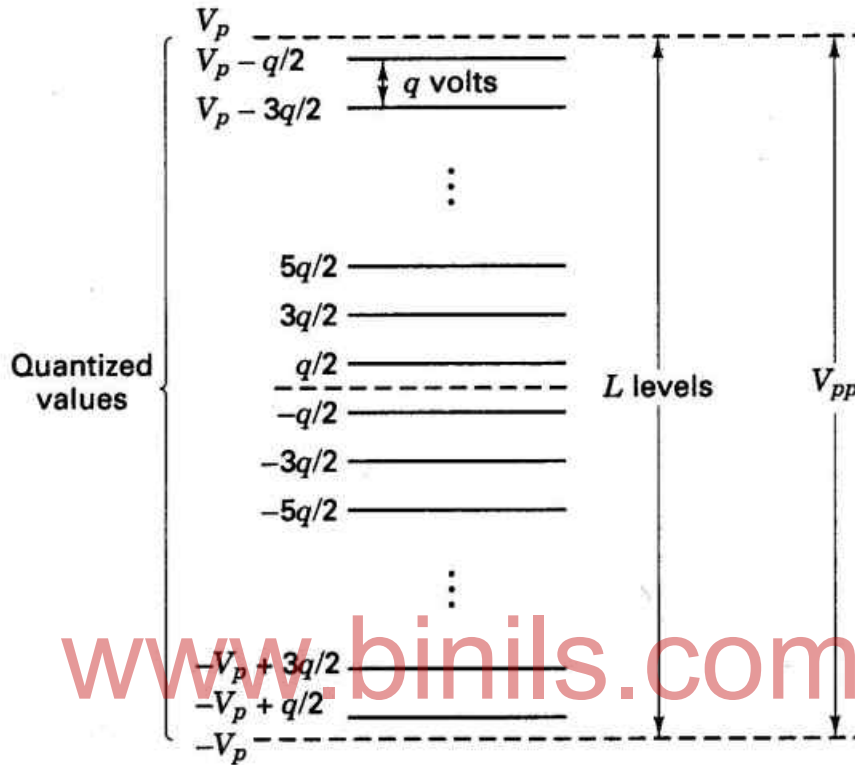
Figure 2.14 (a) Quantization Levels
