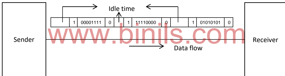
Figure 1.11 Asynchronous transmission
