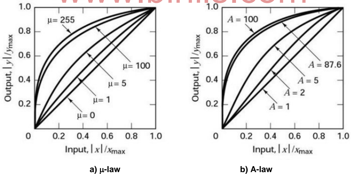
Figure 2.18 Compression Characteristics
