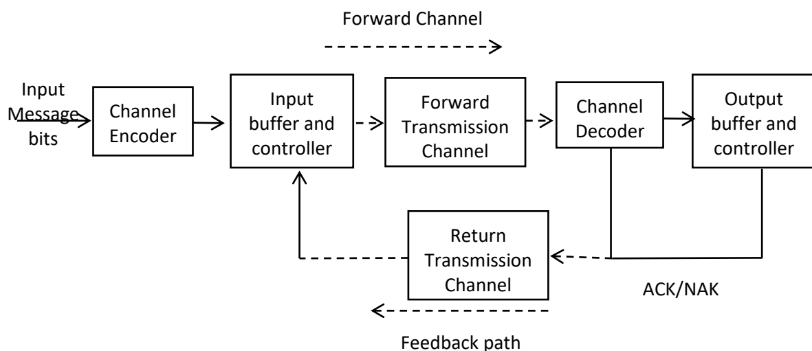
Figure 3.5 : Block diagram of basic ARQ system
