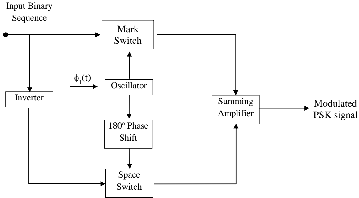
Figure:4.3 (b) Binary PSK modulator
