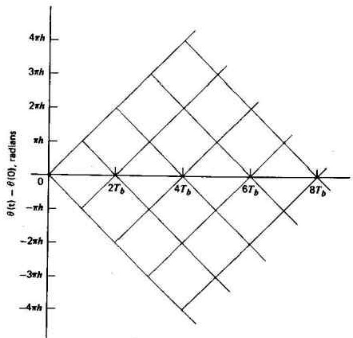
Figure 4.13 Phase Tree
