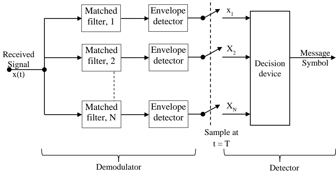
Figure 4.22 Matched filter receiver
