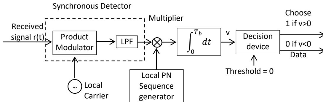
Figure 5.10 DS-BPSK Receiver
