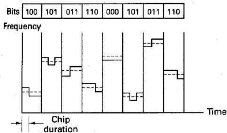
(b) Slow Frequency Hopping
