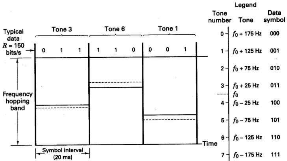
Figure 5.14 Frequency Hopping Example
