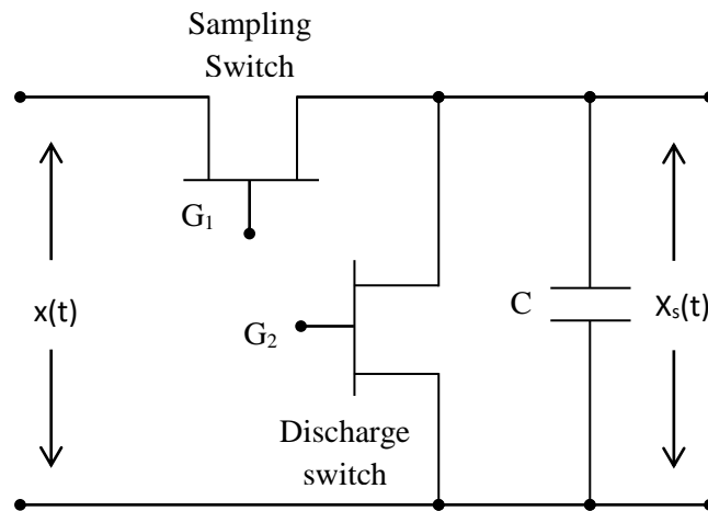
Figure 2.5 Sample and hold circuit for flat top sampling
