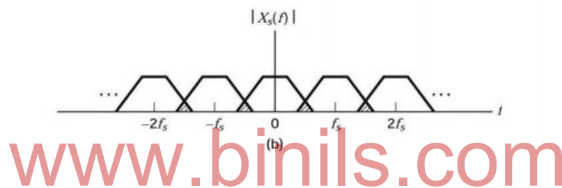
Figure 2.7 Sampled Spectrum for f_s < 2f_m
