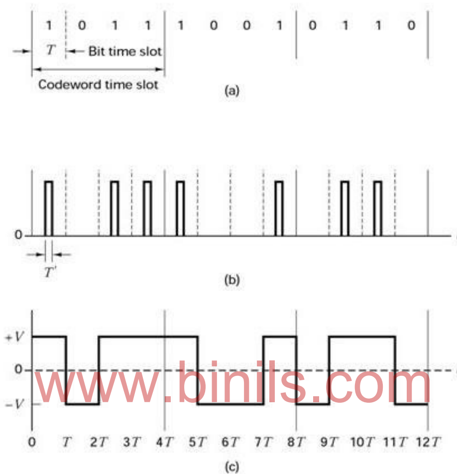
Figure 2.20 Example of waveform representation of binary digits
