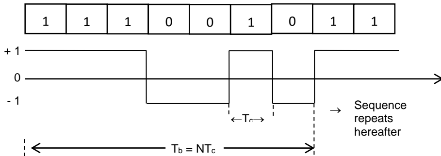
Figure 5.3 PN Sequence waveform
