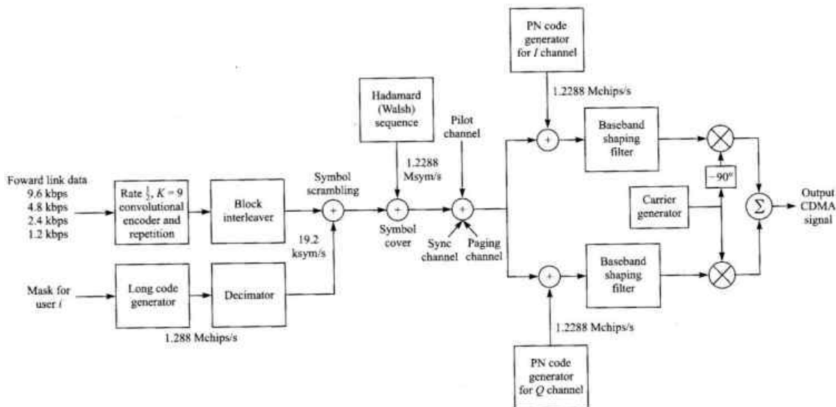
Figure 5.23 IS-95 Forward Link
