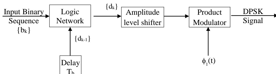
Figure 4.8 DPSK transmitter
