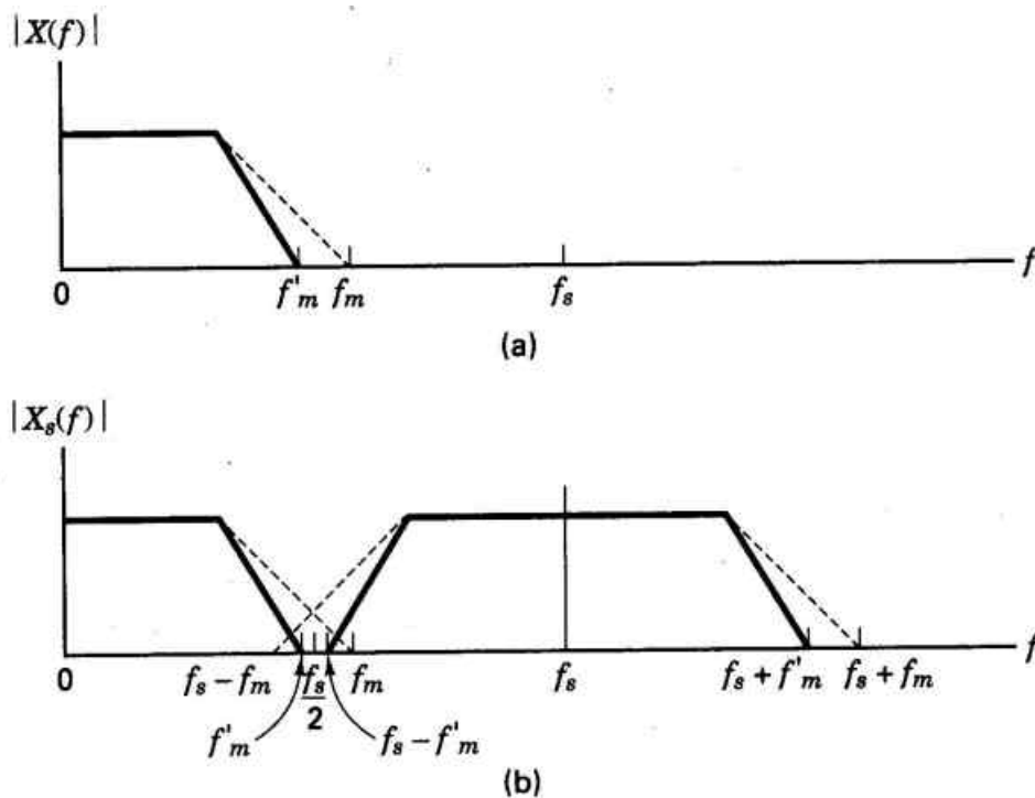
Figure 2.9 Prefiltering
