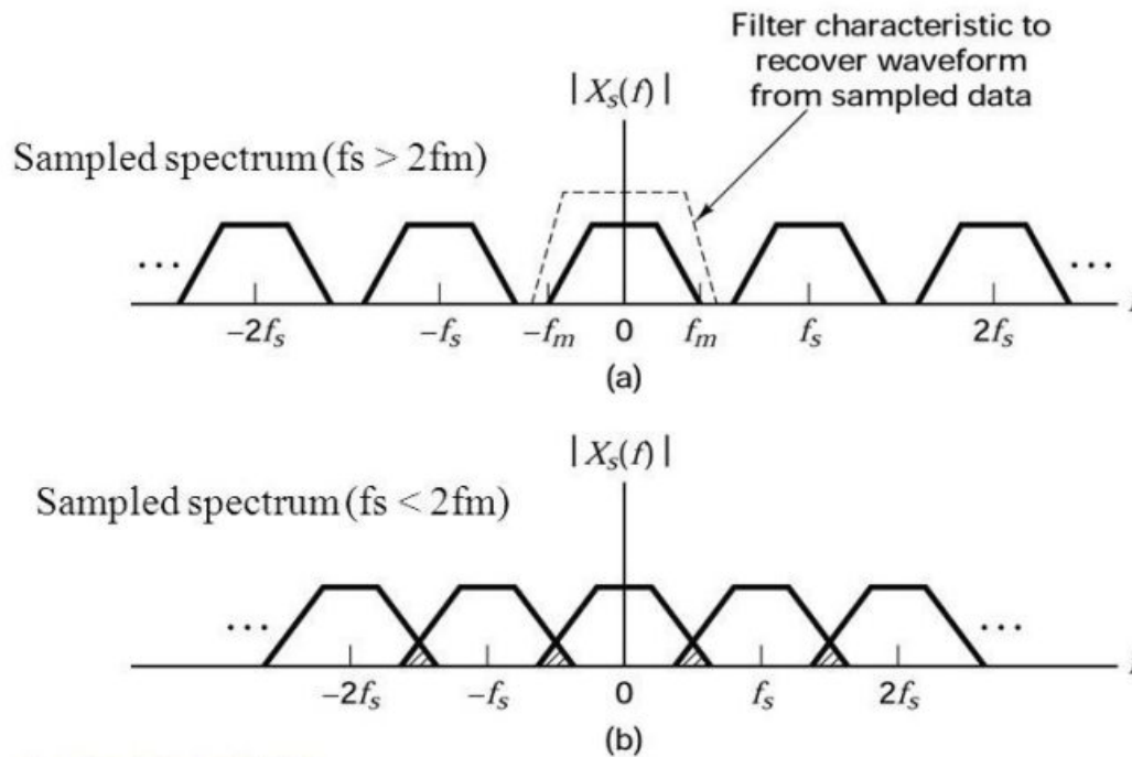
Figure 2.3 Spectra for various sampling rates
