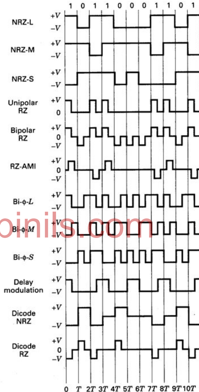
Figure 2.21 Various PCM Waveforms
