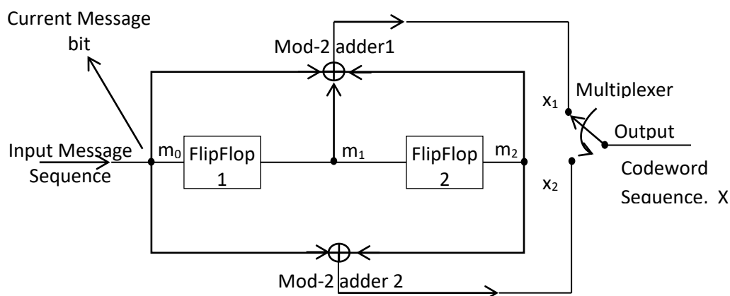
Figure 3.10(a) Convolutional Encoder
