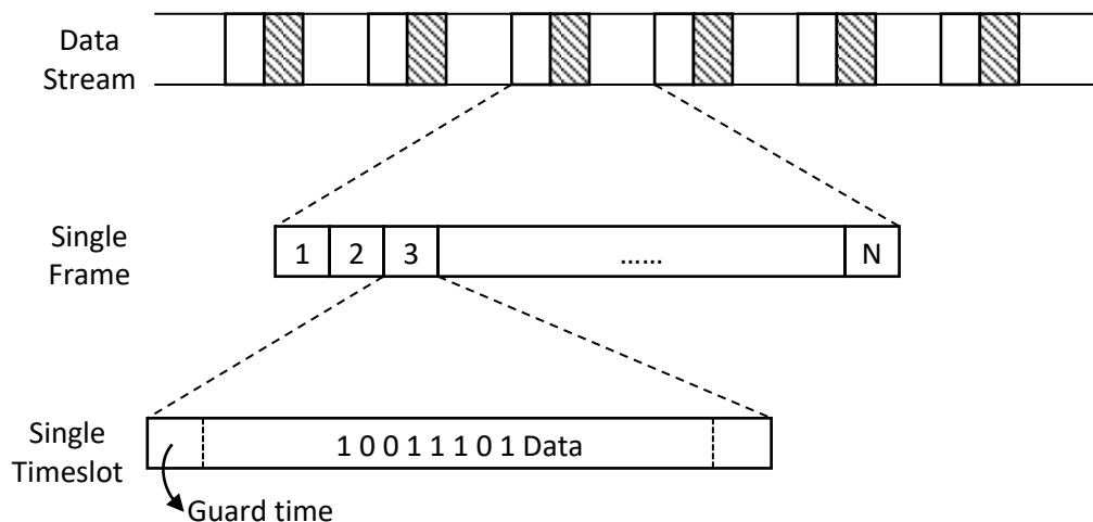
Figure 4.33 TDM Frame structure
