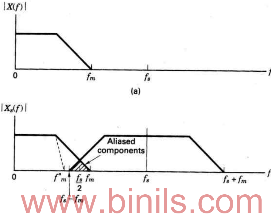
Figure 2.10 Post Filtering
