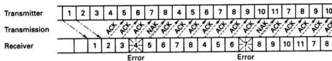
(b) Go back-N ARQ
