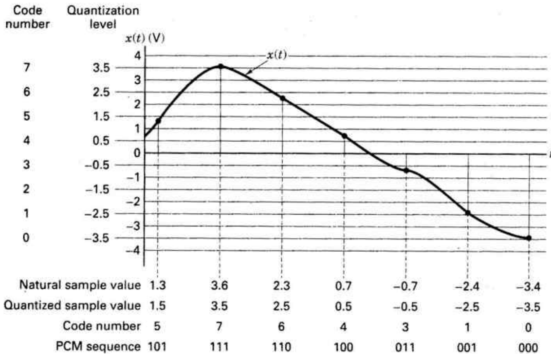
Figure 2.14 (b) Pulse Code Modulation
