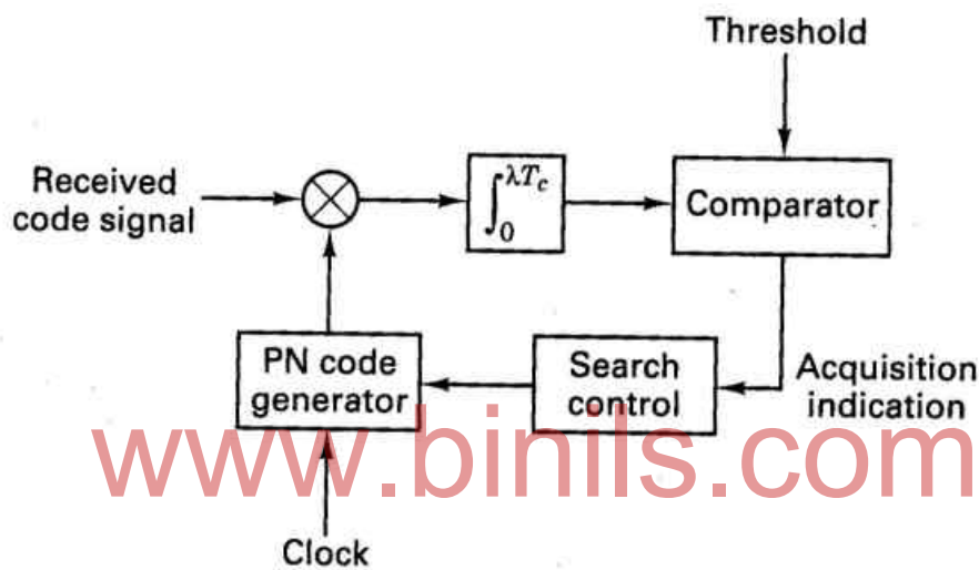
Figure 5.19 Direct Sequence spread spectrum systems – Serial Search Acquisition
