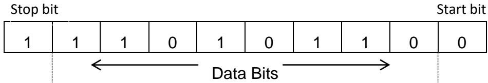
Figure 1.10 Data bytes
