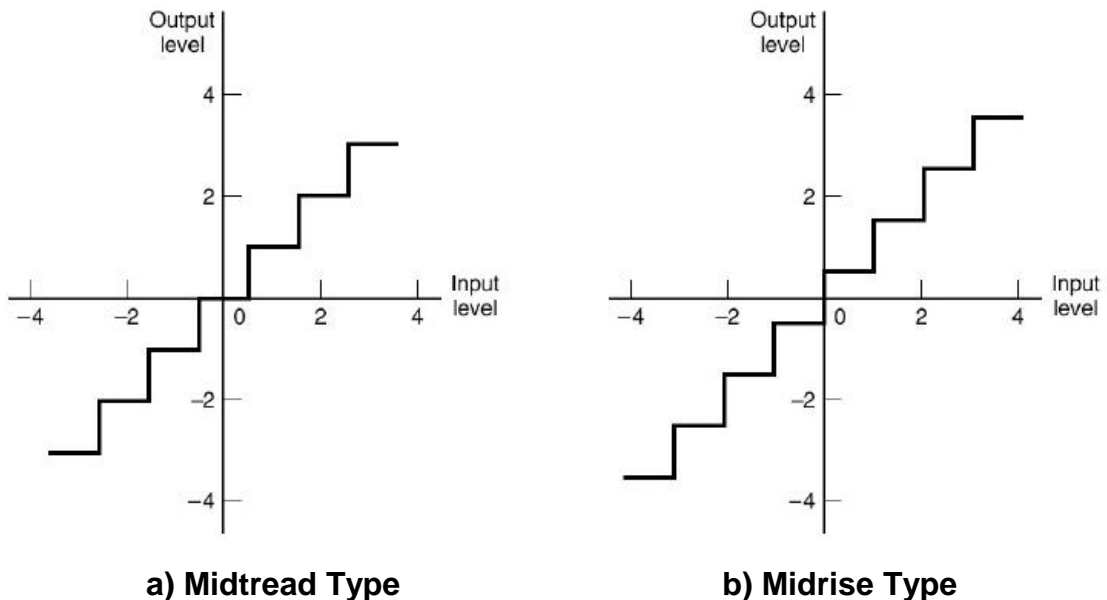
Figure 2.15 Two types of Uniform Quantization
