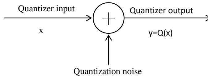
Figure 2.12 Quantizer
