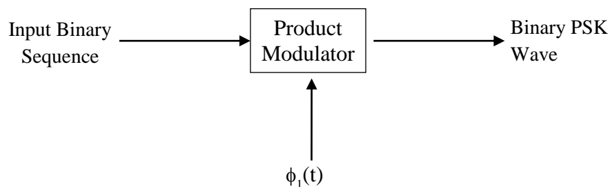
Figure 4.3(a) Binary PSK transmitter
