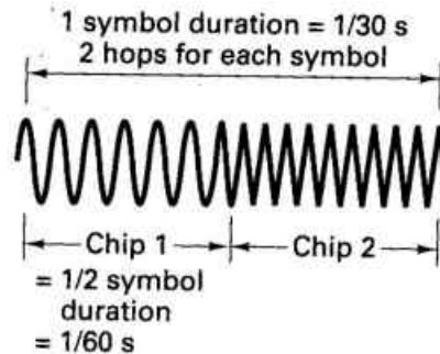
(a) Fast frequency hopping
