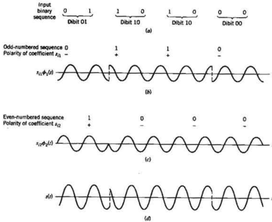
Figure 4.10 QPSK waveforms
