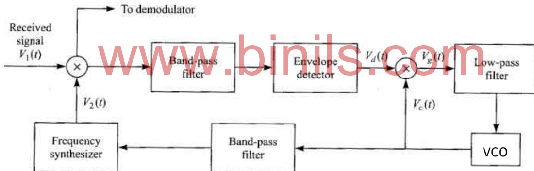
Figure 5.22 Tracking loop for FH signals
