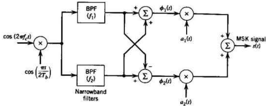
Figure 4.15 Block diagram of MSK transmitter communication system
