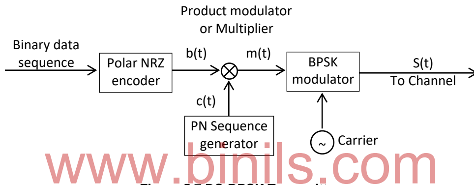
Figure 5.7 DS-BPSK Transmitter
