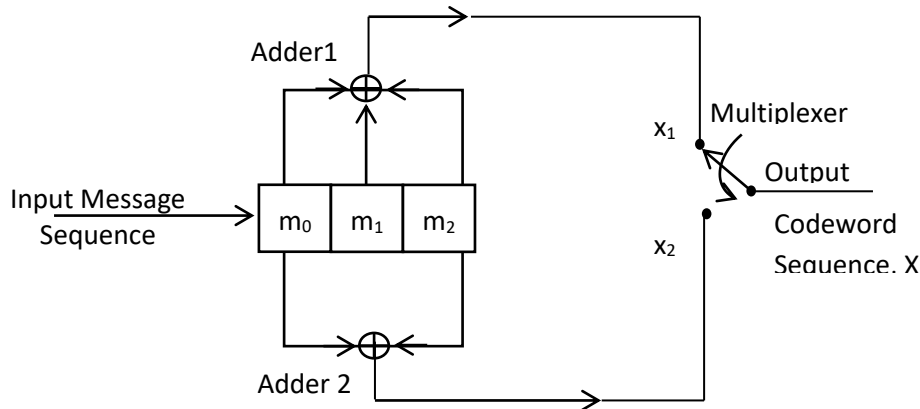
Figure 3.10(b) Convolutional Encoder redrawn alternatively
