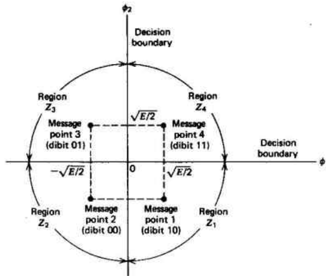
Figure 4.12 Signal space diagram for coherent QPSK system
