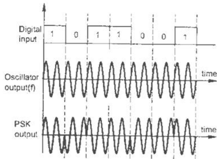
Figure 4.4 - Waveforms for BPSK
