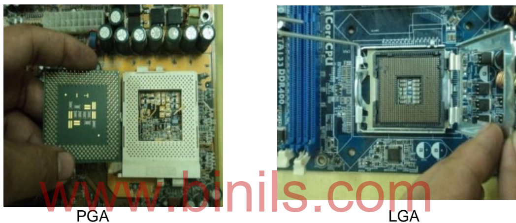
Figure 1.2 PGA and LGA Sockets
