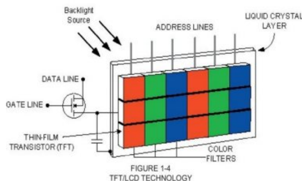
Figure 3.5 TFT Glass
