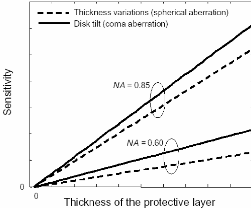
www.binils.com Figure 2.11 Sensitivity of the Spot
