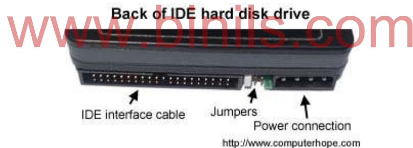
Figure 1.7 Jumpers
