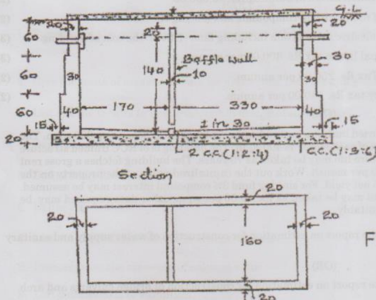
Figure - 2 (All Dimensions are in mm)
